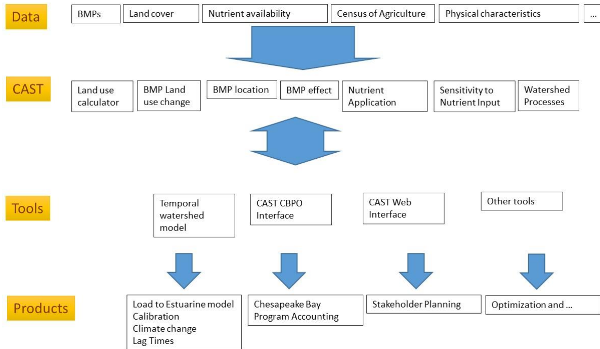
Figure 1-5: Phase 6 software structure
